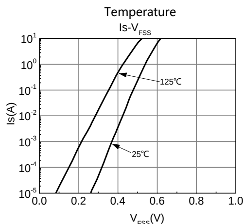
Figure 6: Forward Source to Source Characteristics
