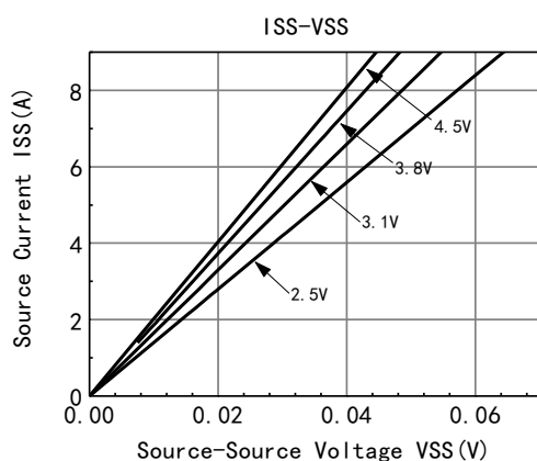
Figure 1: On-Region Characteristics
