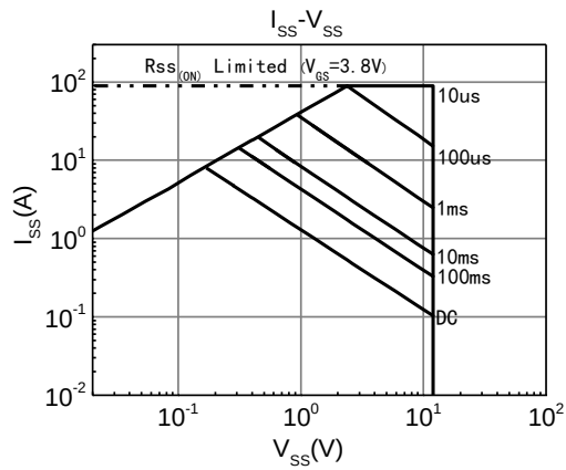
Figure 9: Safe Operating Area
